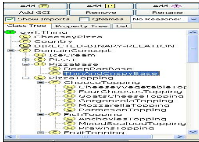
Fig. 4: Extracting the Class ThinAndCrispyBase for SubOntology
