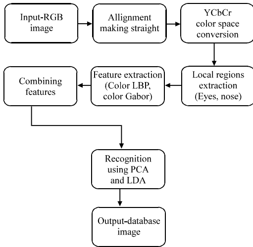
Fig. 5: System block diagram of color FR framework based on color local texture features
