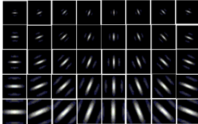
Fig. 2: The real part of the Gabor filters with five frequencies and eight orientations for \omega_{max} = \pi/2 , the row corresponds to different frequency \omega_m , the column corresponds to different orientation \theta_n
