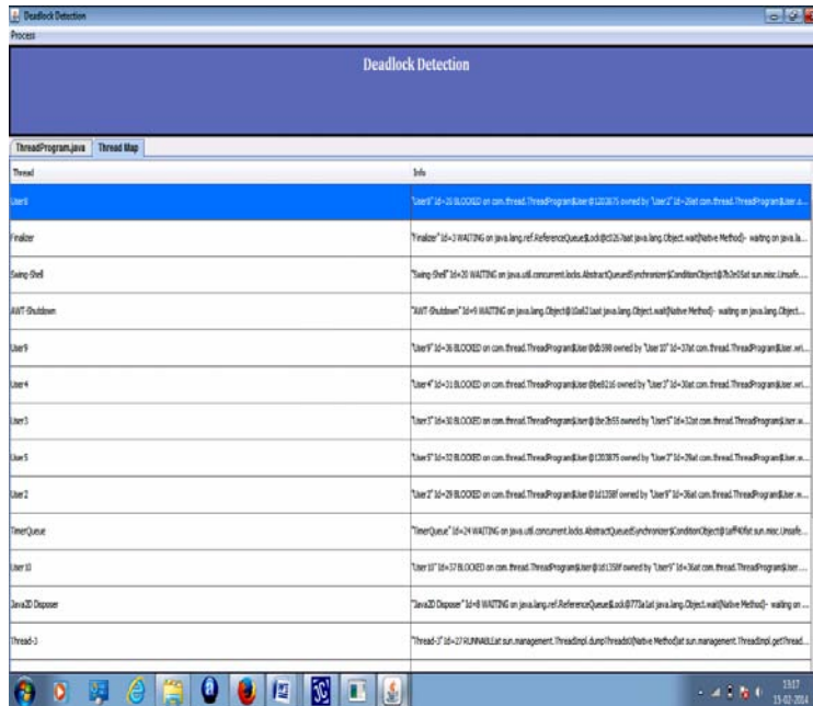
Fig. 2: Deadlock detection window with threadmap
