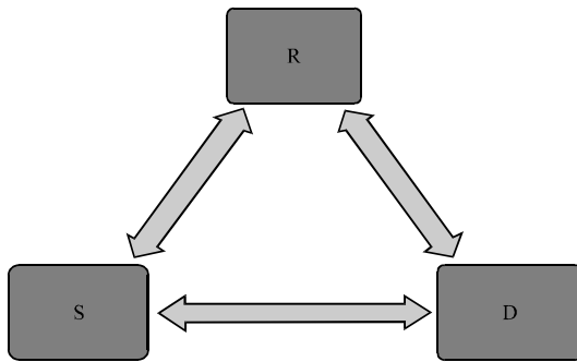
Fig. 1: Relay channel
