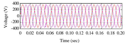
Fig. 17: Load voltage after swell mitigation by UPQC with NN controller
