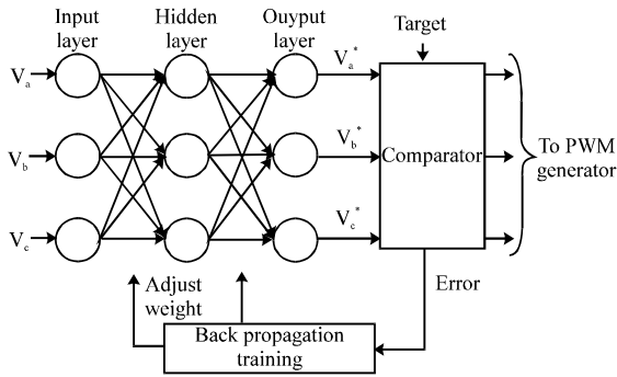
Fig. 4: Neural network controller
