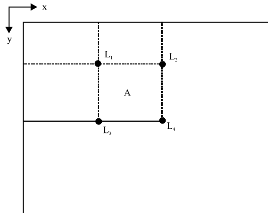
Fig. 6: Calculating figure using the integral image
