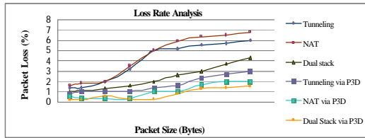
Fig. 7: Loss rate analysis
