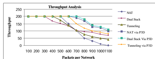
Fig. 4: Throughput analysis
