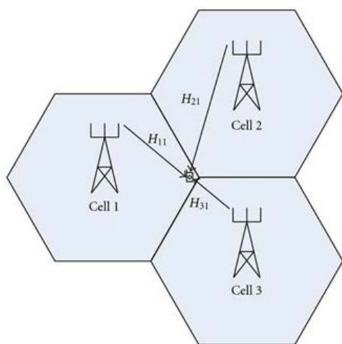
Fig. 4: CoMP Transmission
