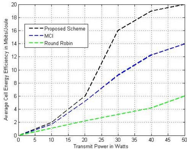
Fig. 11: Comparison of average cell energy efficiency for various transmission power
