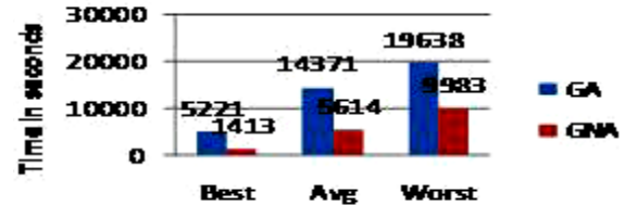
Fig. 14: Execution of P21 in tight time schedule
