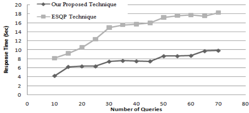
Fig. 9: Measuring the query throughput
