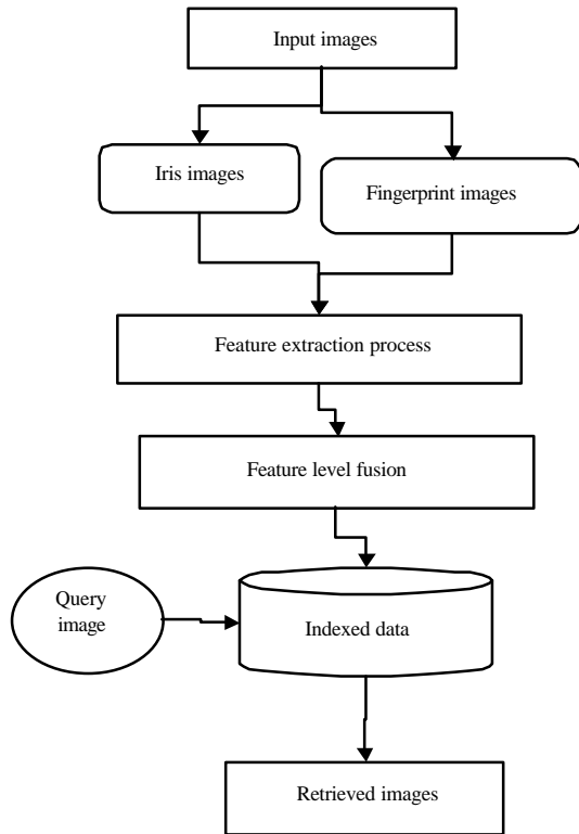
Fig. 1: Architecture for TMB-CBIR approach
