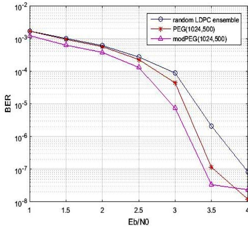
Fig. 2: BER vs Eb/No for random LDPCs ensemble and PEG with modPEG
