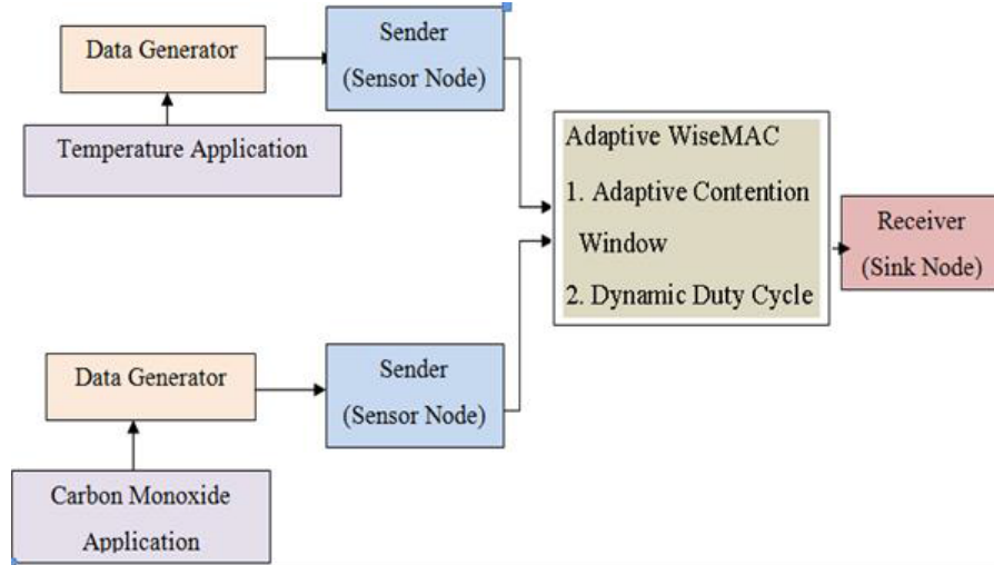
Fig. 3: AWiseMAC architecture
