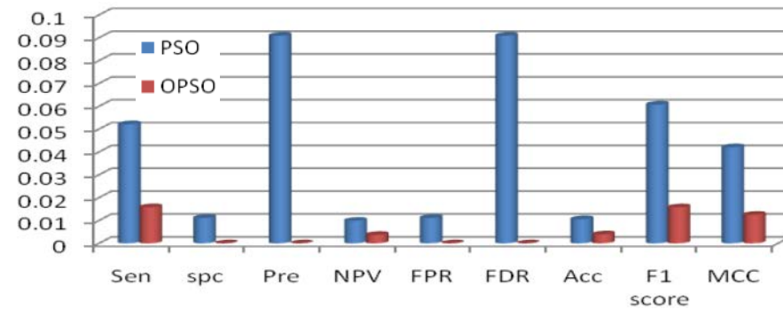
Fig. 10: Comparison of performance measures for standard deviation by PSO and OPSO
