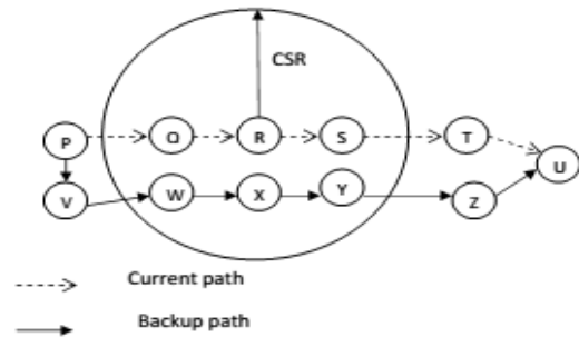
Fig. 3: Calculation of Contention Difference (CD)
