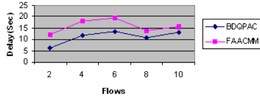
Fig. 6: Flows vs. delay
