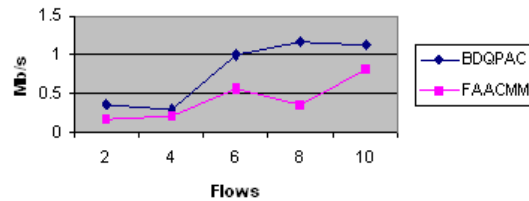
Fig. 7: Flows vs. received bandwidth
