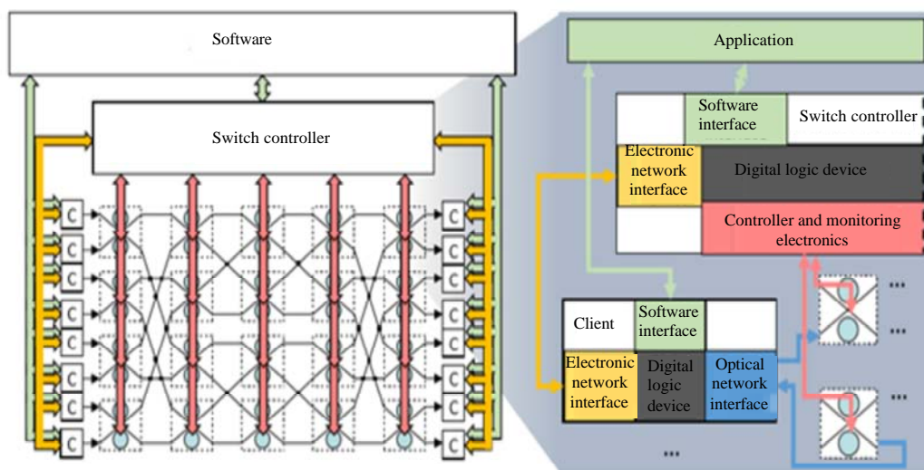
Fig. 6: Silicon photonic computing architecture applicable to Li-Fi backbone network
