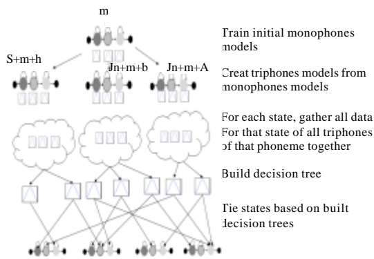
Fig. 2: The detailed process of phonetic decision tree state tying
