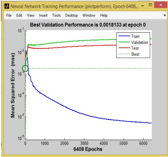
Fig. 6: The graphical result showing the best validation performance
