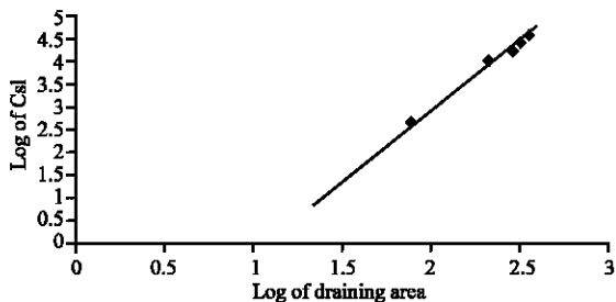
Fig. 4: Plot of logarithm of Cumulative stream length (Csl) to logarithm of drainage area for river Gongola in km
