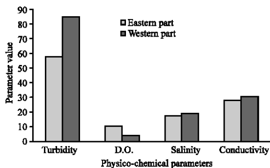
Fig. 2: Mean turbidity, D.O, salinity and conductivity in the two parts of the Lagoon
