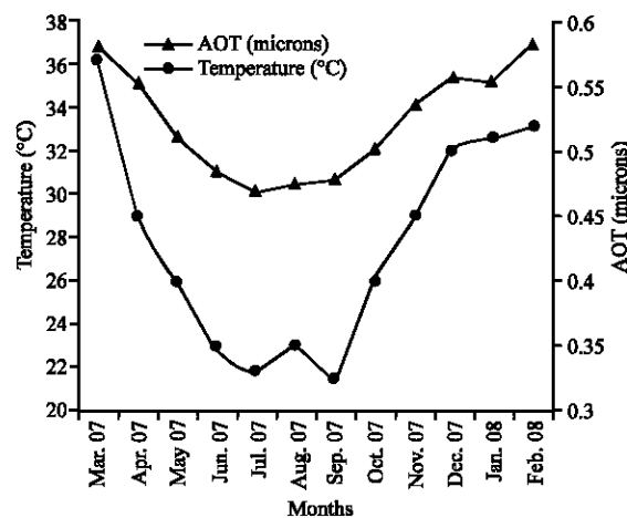
Fig. 2b: Temperature and AOT in Nigeria between March 2007 and February 2008
