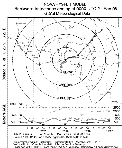
Fig. 8a: Backward trajectory analysis (96 h) at three altitudes, start of run at 00:00, 21 Apr 2007
