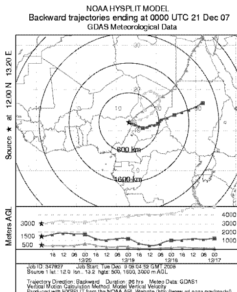
Fig. 7b: Backward trajectory analysis (96 h) at three altitudes, start of run at 00:00, 21 Dec 2007
