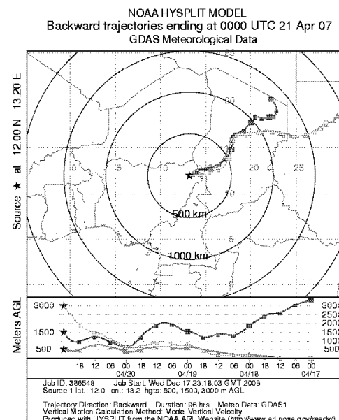
Fig. 3b: Backward trajectory analysis (96 h) at three altitudes, start of run at 00:00, 21 Apr 2007
