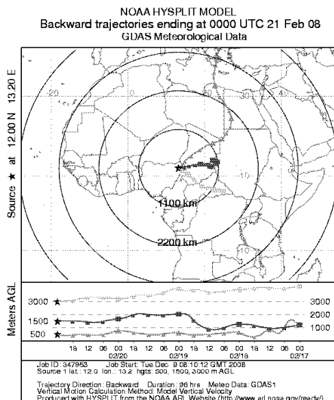
Fig. 8b: Backward trajectory analysis (96 h) at three altitudes, start of run at 00:00, 21 Feb 2008
