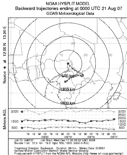
Fig. 5b: Backward trajectory analysis (96 h) at three altitudes, start of run at 00:00, 21 Aug 2007
