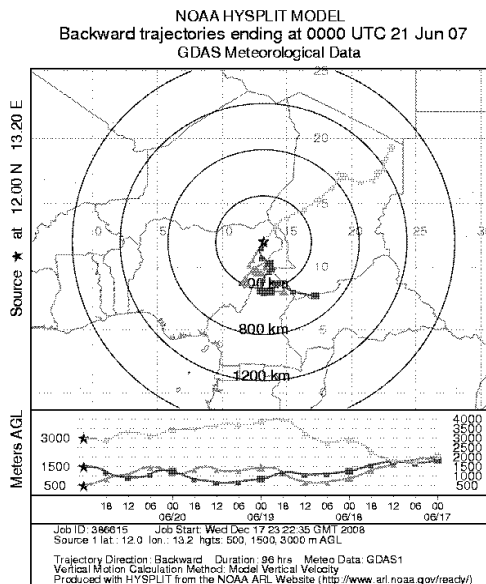
Fig. 4b: Backward trajectory analysis (96 h) at three altitudes, start of run at 00:00, 21 Jun 2007
