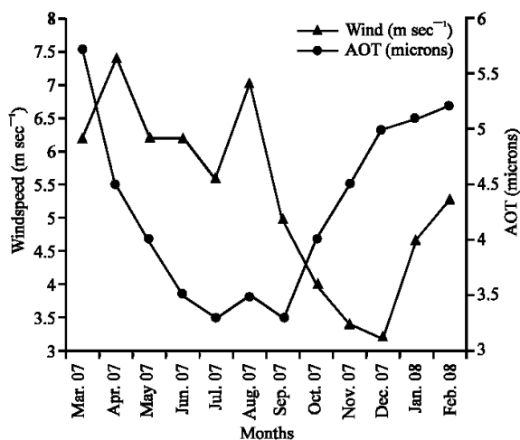
Fig. 2c: Wind speed and AOT in Nigeria between March 2007 and February 2008
