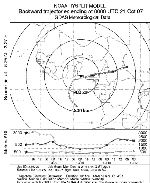
Fig. 6a: Backward trajectory analysis (96 h) at three altitudes, start of run at 00:00, 21 Oct 2007
