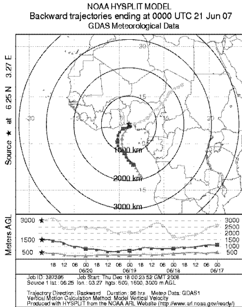
Fig. 4a: Backward trajectory analysis (96 h) at three altitudes, start of run at 00:00, 21 June 2007
