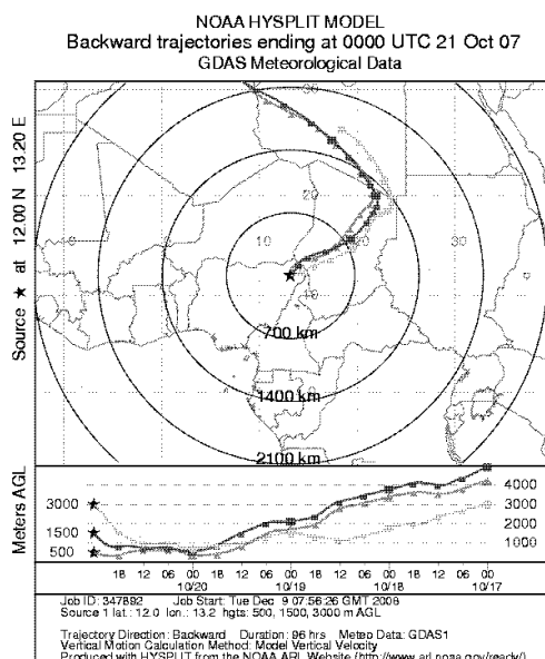
Fig. 6b: Backward trajectory analysis (96 h) at three altitudes, start of run at 00:00, 21 Oct 2007
