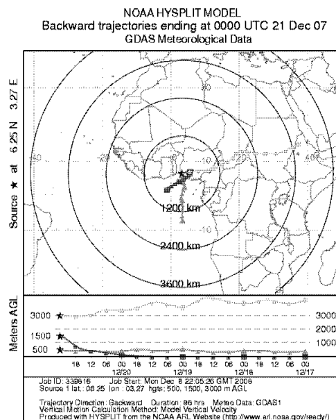
Fig. 7a: Backward trajectory analysis (96 h) at three altitudes, start of run at 00:00, 21 Dec 2007
