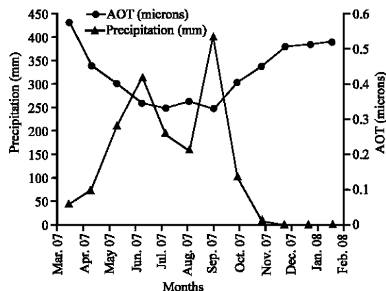
Fig. 2a: Precipitation and AOT in Nigeria between March 2007 and February 2008
