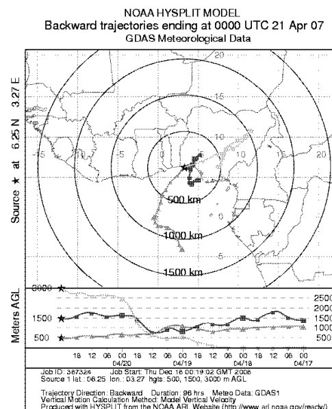
Fig. 3a: Backward trajectory analysis (96 h) at three altitudes, start of run at 00:00, 21 Apr 2007
