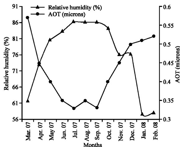
Fig. 2d: Relative humidity and AOT in Nigeria between March 2007 and February 2008
