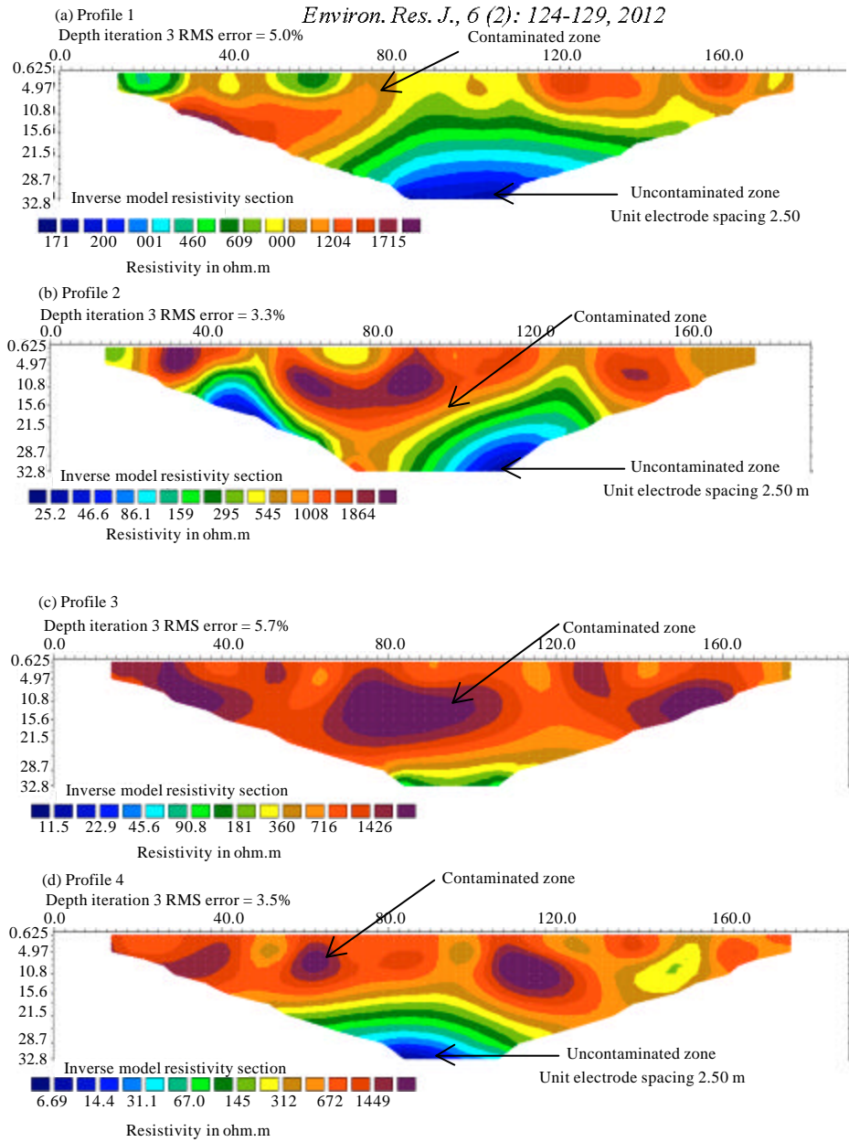
Fig. 2a-d: Inverted resistivity sections of the profiles 1-4
