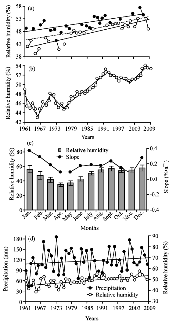
Fig. 7: a) The inter-annual variation of air humidity during 1961-2009; b) Periodic variation of air humidity during 1961-2009; c) Monthly variation of air humidity during 1961-2009 and d) The correlation between air humidity and the annual precipitation during 1961-2009
