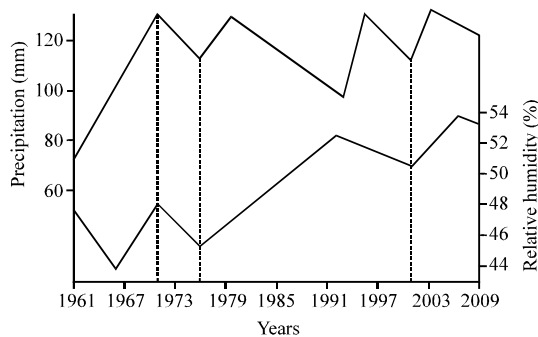
Fig. 9: The variation phases of air humidity and precipitation during 1961-2009 were not completely corresponded
