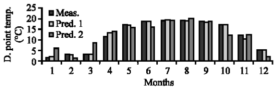
Fig. 3: Column graph showing Meas. and Pred. 1 and 2 dew point temp. value for Jos
