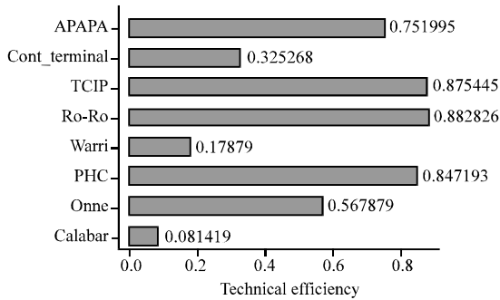
Fig. 1: Distribution of efficiency values by respective ports (Efficiency analysis of Nigeria’s sea ports)
