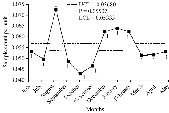
Fig. 6: U chart of total defect
