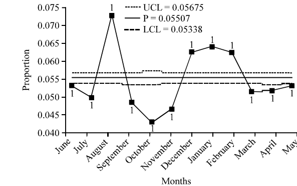
Fig. 5: P chart of total defect
