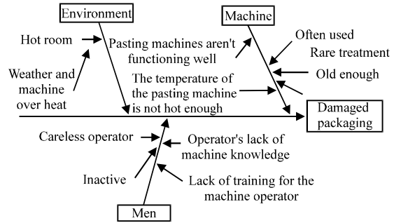
Fig. 8: Damaged packaging cause and effect diagram
