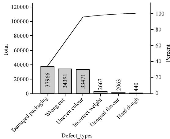
Fig. 7: Defect types Pareto diagram
