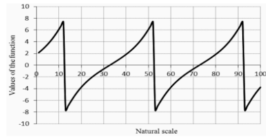
Fig. 16: “Sawtooth wave” function graph expressed by Eq. 11
