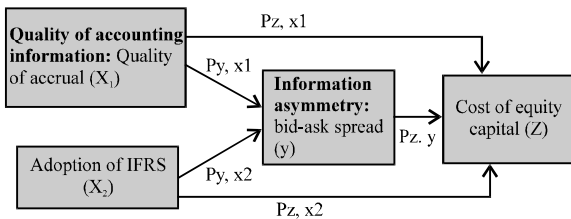
Fig. 1: Model of path analysis test
