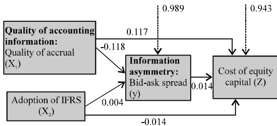
Fig. 2: Result of path analysis test
