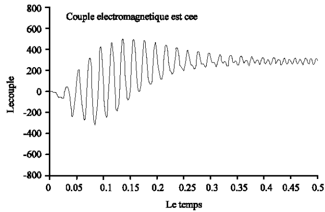
Fig. 5: Electromagnetic torque
