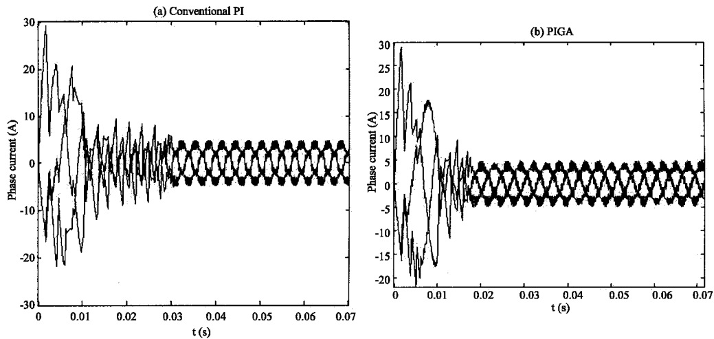
Fig. 12: Phase's currents response for T_m = 4 Nm
