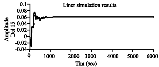
Fig. 19: System response for \Delta_{15} with PSS in Machine 4 and 2
