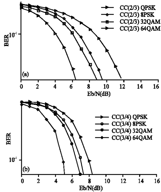
Fig. 3: System performance under different modulation schemes for RS (255, 239, 8) concatenated with CC (code rate of 2/3, 3/4)
