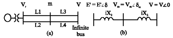
Fig. 1: A single-machine infinite bus system: a) single-line diagram and b) equivalent circuit
