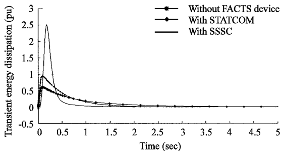
Fig. 11: Transient energy (pu) vs. time (sec) for gain K = 1.5
