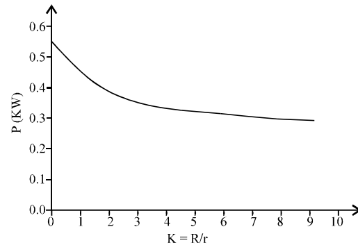
Fig. 4: Dependence of the power in shaft end of the engine according to the degree rotor asymmetry
