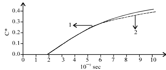
Fig. 6: Mechanical characteristics; 1) calculated and 2) experimental cage engine at the time of a combination of electric failures (rupture of 15 bars to the rotor and a phase with the stator)
