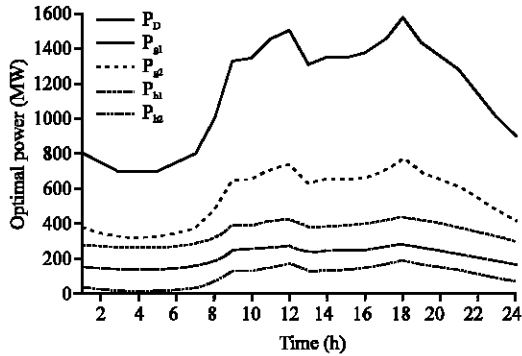
Fig. 7: Optimal power generation schedule using genetic algorithm
