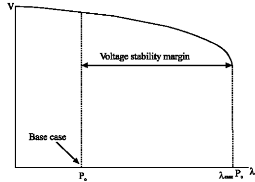
Fig. 1: P-V curve or nose-curve
