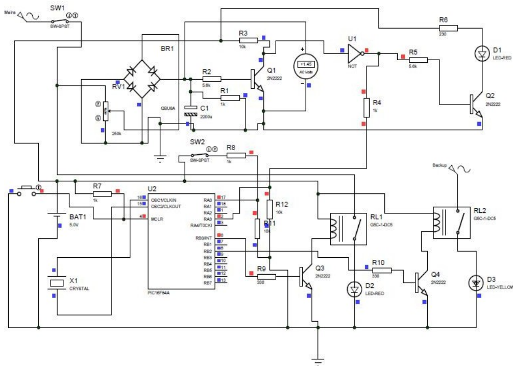
Fig. 2: Complete schematic diagram of \mu\text{C} based automatic electrical mains changeover system
