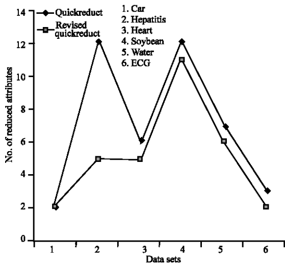
Fig. 2: Performance analysis of the Quickreduct and the Revised Quickreduct(Mean Imputation1)
