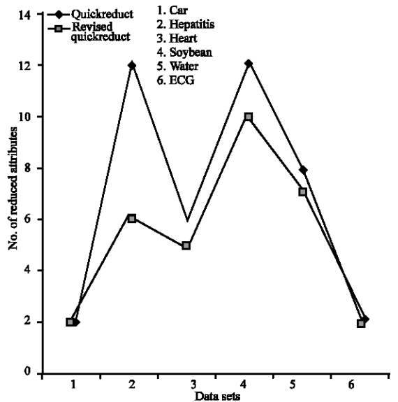
Fig. 5: Performance analysis of the Quickreduct and the Revised Quickreduct(Mode)
