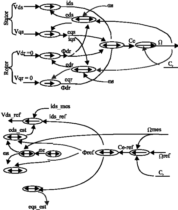
Fig. 7: CIG representation of induction machine
