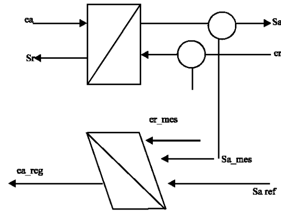
Fig. 4: Inversion of adaption elemnet
