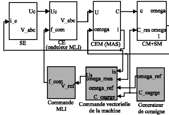
Fig. 8: The control structure of induction machine
