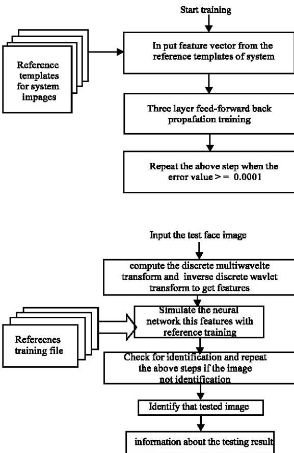
Fig. 7: The neural network classifier architecture for image Identification
