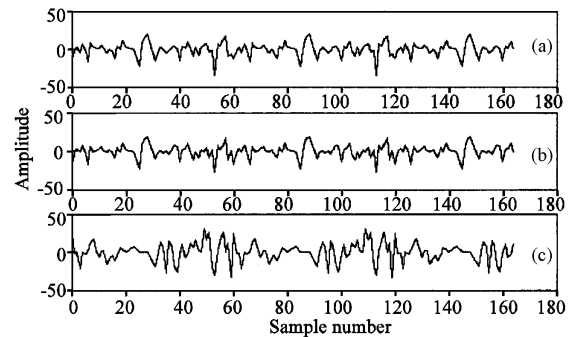
Fig.10: (a) EEG signal (b) Estimated combined artifacts present in the EEG signal (c) Estimated EEG signal after removing the artifact
