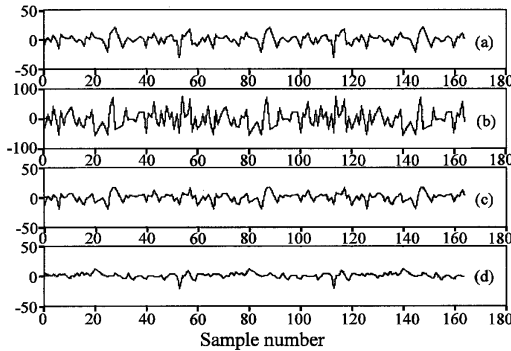
Fig. 7: (a) EEG signal (b) EOG Left artifact (c) Estimated EOG Left present in the EEG signal (d) Estimated EEG signal after removing the artifact
