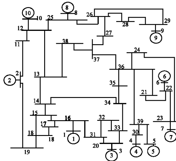
Fig. 2: Configuration of new England 39 bus system
