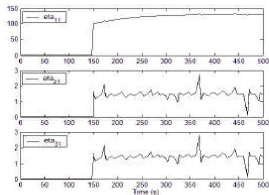
Fig. 11: Trends of decision functions under h_1 sensor failure condition with set point set at 10 cm
