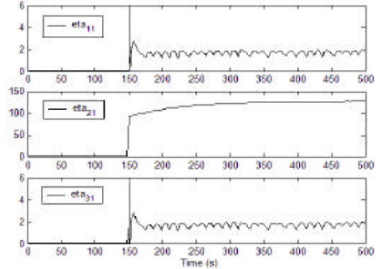
Fig. 15: Trends of decision functions under h_2 sensor failure condition with set point set at 10 cm
