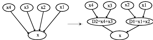
Fig. 4: Graph for risk factors representational fragment
