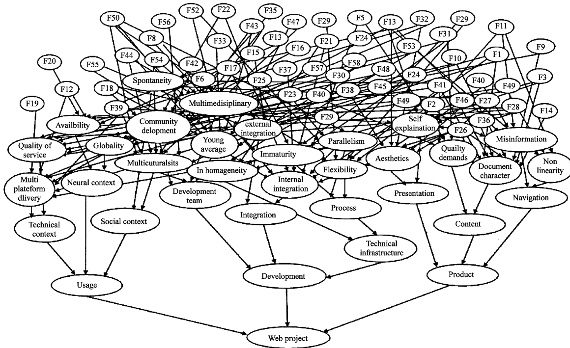
Fig. 3: Bayesian network graph
