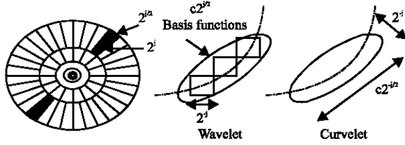
Fig. 1: Curvelet transform (Candes et al. , 2006)
