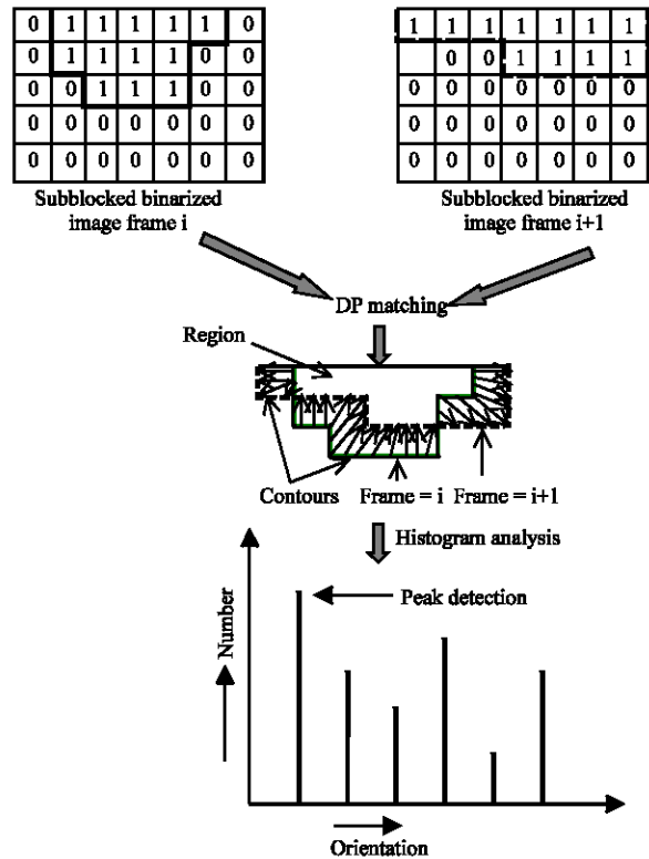
Fig. 2: Procedural steps for detection of global smoke direction
