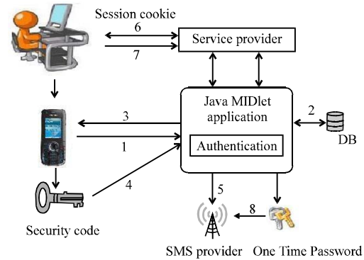
Fig. 3: Proposed layout of authentication protocol
