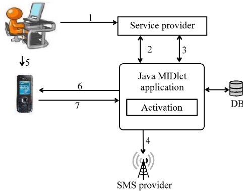
Fig. 2: Proposed layout of activation protocol
