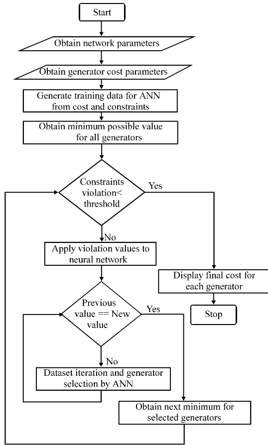
Fig. 4: Flow chart of ANN-GD-OPF
