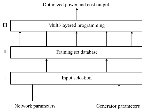
Fig. 1: The conceptual diagram of learning model for MLP
