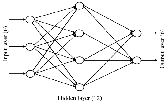
Fig. 2: Topology of a three layered MLP
