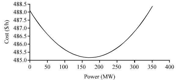
Fig. 6: Cost power curve of Generator G1
