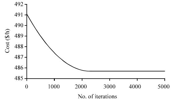
Fig. 5: Cost convergence in gradient descent (Generator G1)
