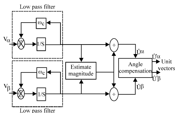
Fig. 2: Block diagram of unit vector generation
