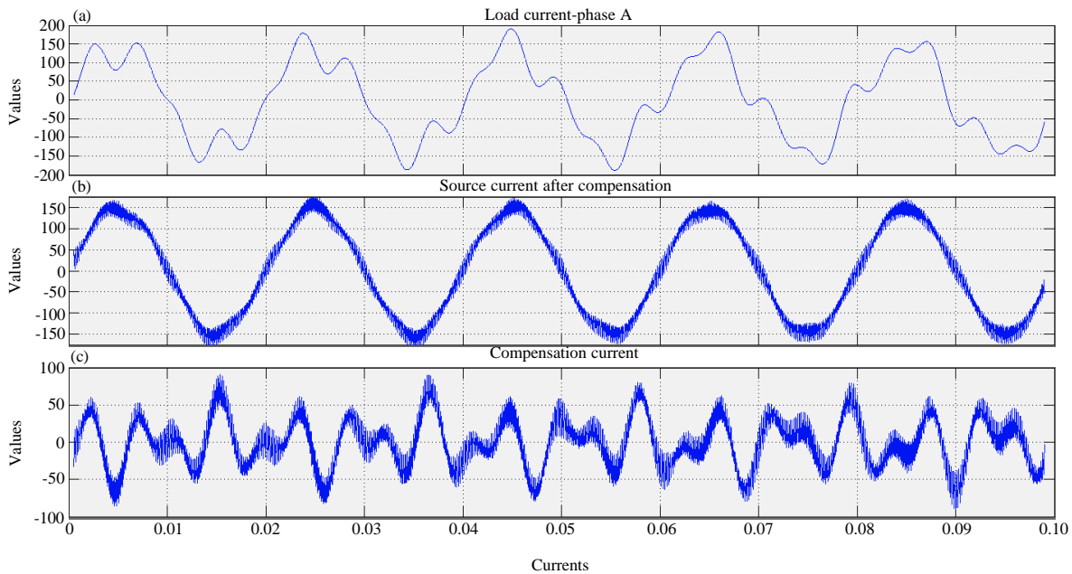
Fig. 6: MATLAB/SIMULINK result of phase A showing the: a) load current for 100 kVAR load; b) source current after compensation and c) compensation current injected by the filter into to the point of common coupling
