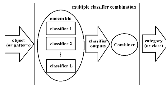
Fig. 1: Multiple classifier combination architecture
